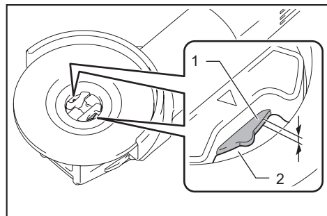
► 1. Surface du support 2. Surface de la meule X-LOCK
