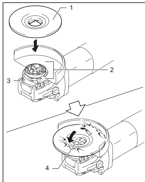
► 1. Meule X-LOCK 2. Support 3. Surface du flasque 4. Loquet
